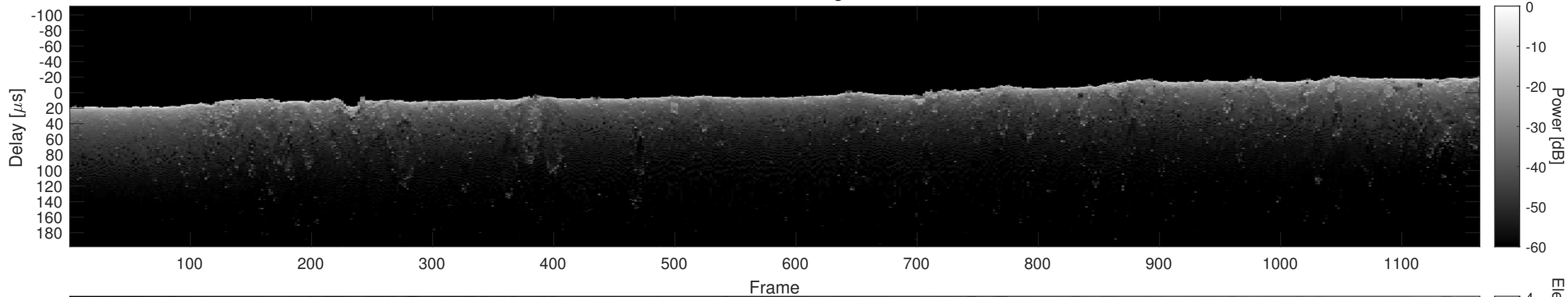
Orbit 21830, Cluttergram
