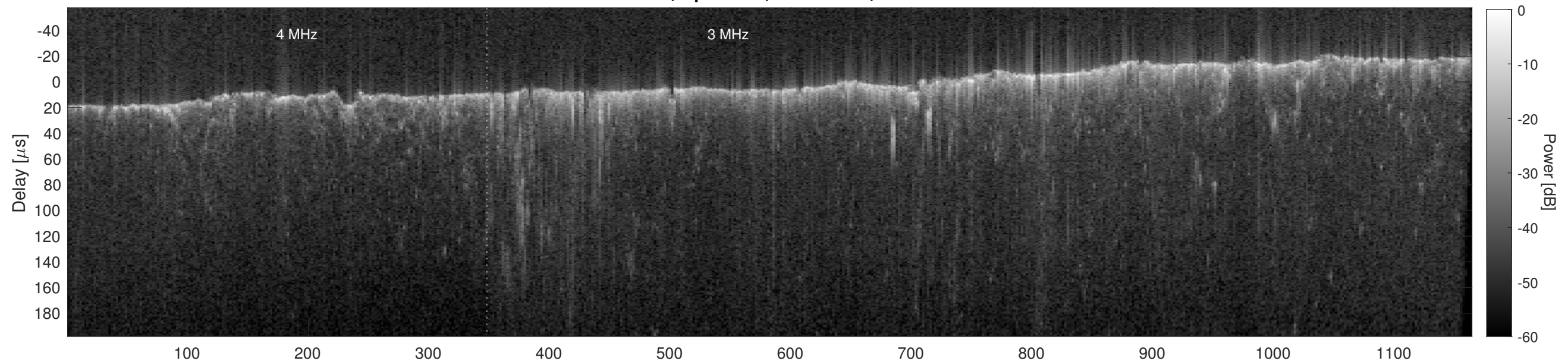
Orbit 21830, Cluttergram
