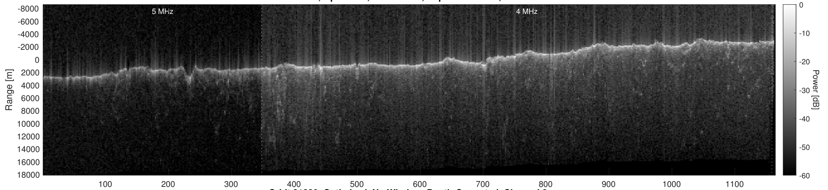
Orbit 21830, Optimized, No Window, Depth-Corrected, Channel 2
