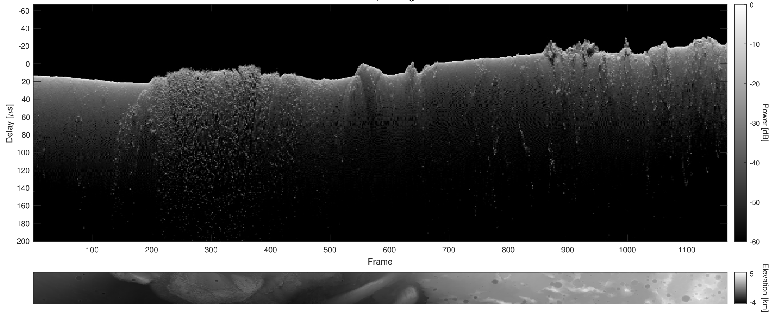
Orbit 21835, Cluttergram
