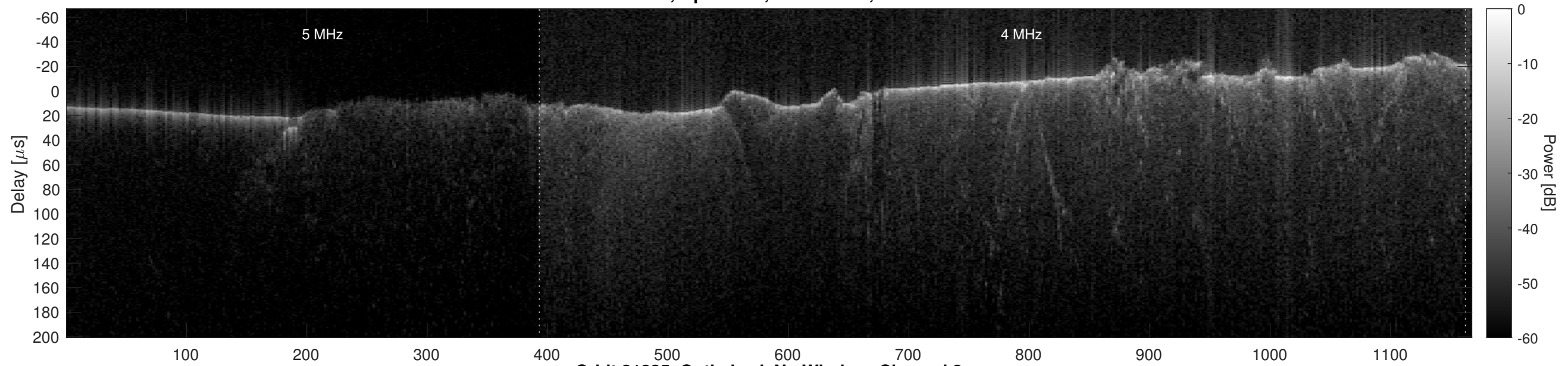
Orbit 21835, Optimized, No Window, Channel 2
