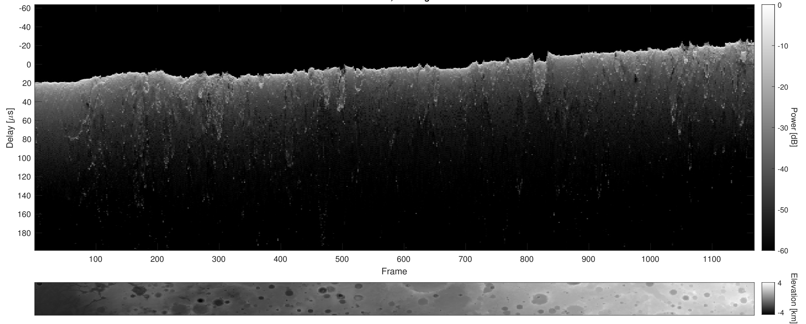
Orbit 21837, Cluttergram
