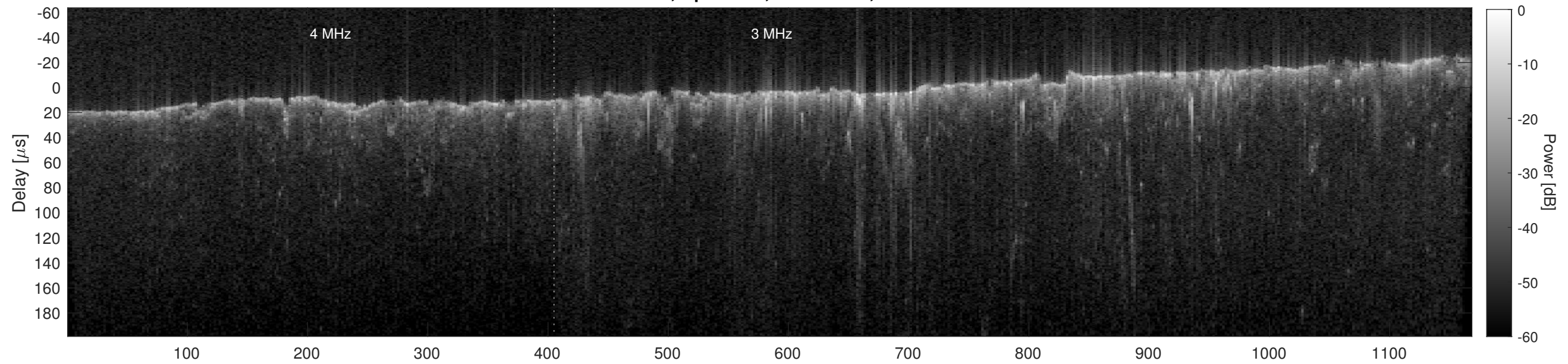
Orbit 21837, Cluttergram
