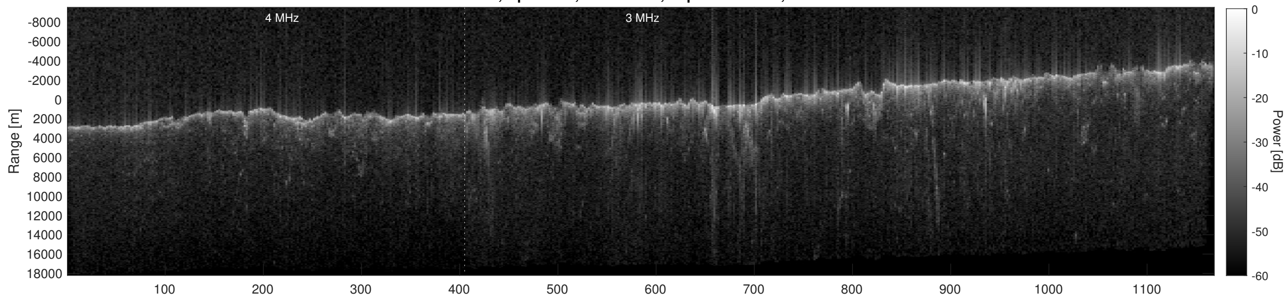
Orbit 21837, Depth-Corrected Cluttergram
