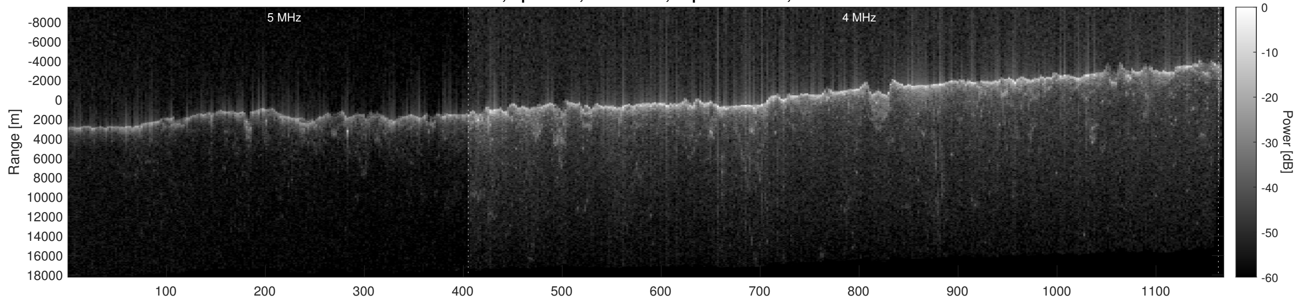
Orbit 21837, Optimized, No Window, Depth-Corrected, Channel 2
