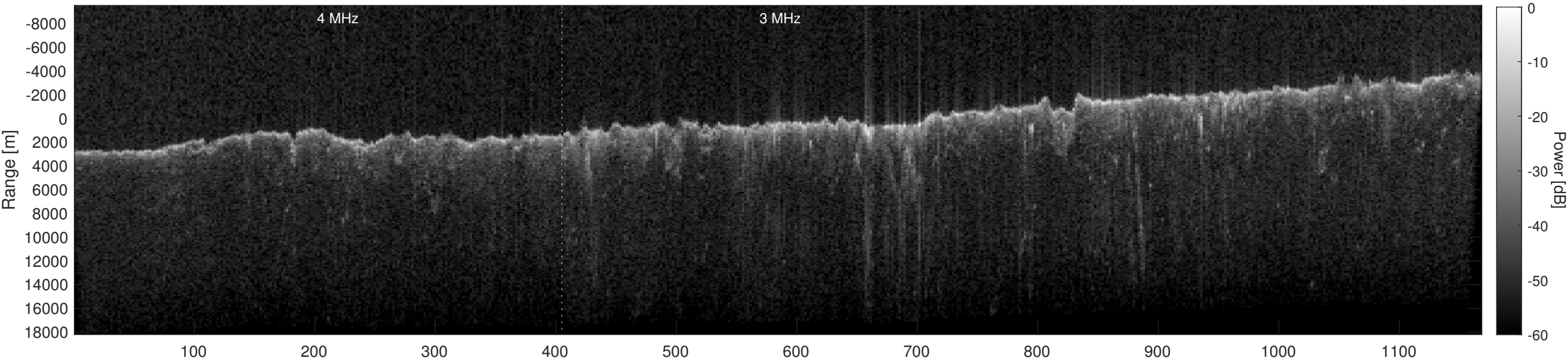
Orbit 21837, Depth-Corrected Cluttergram
