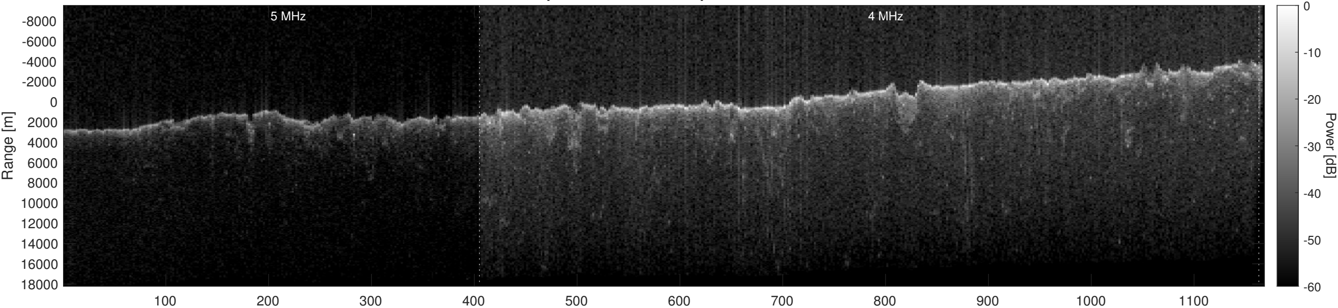
Orbit 21837, Optimized, Window, Depth-Corrected, Channel 2
