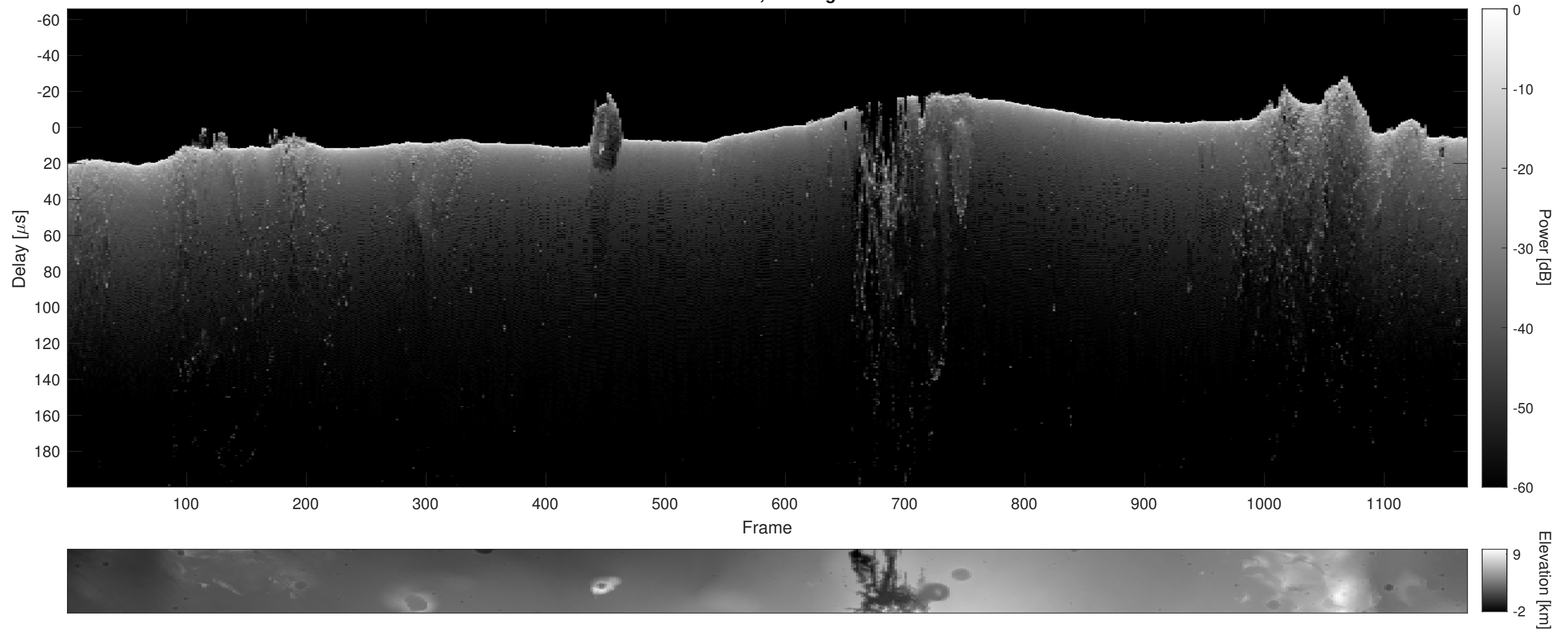
Orbit 21838, Cluttergram
