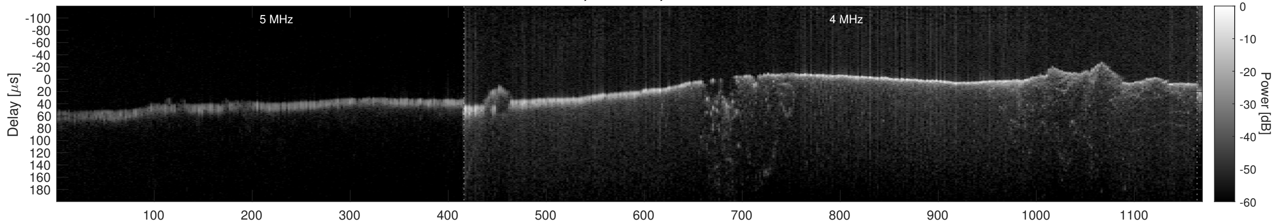
Orbit 21838, Window, Channel 1, Chapman
