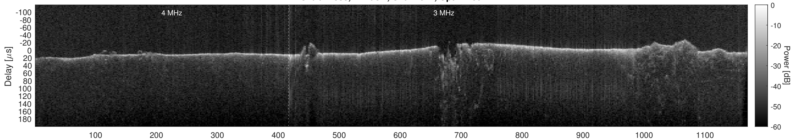
Orbit 21838, Cluttergram
