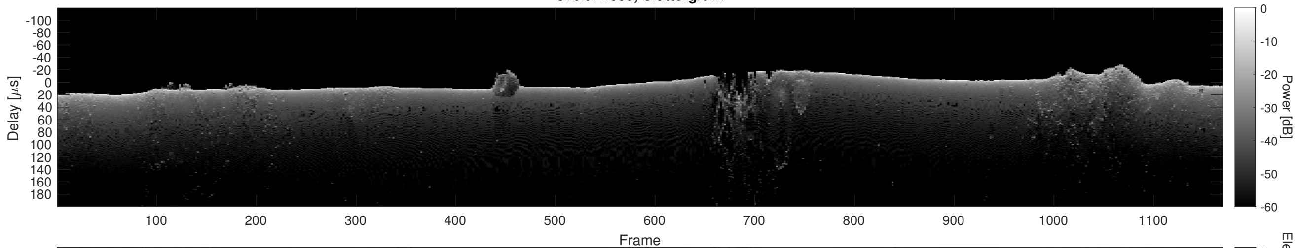
Orbit 21838, Cluttergram
