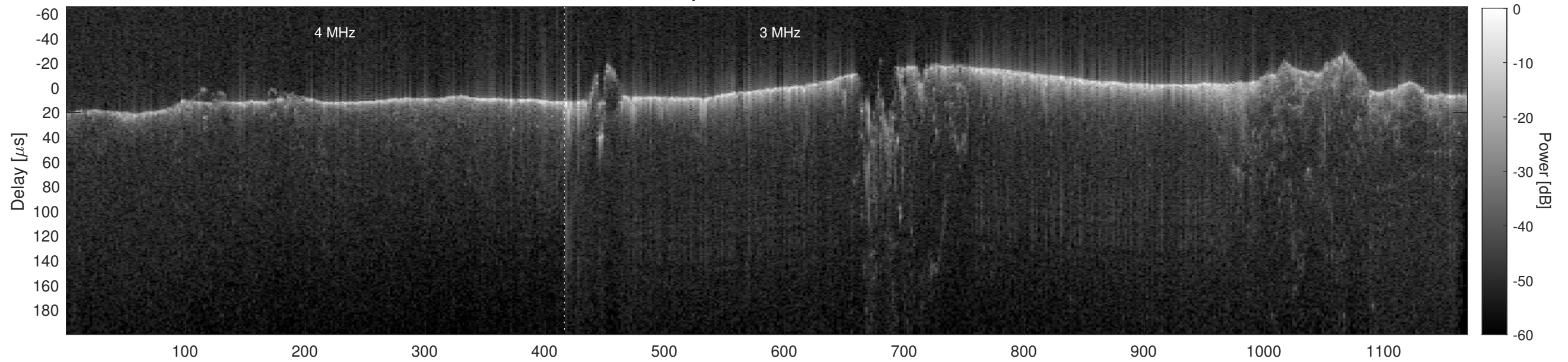
Orbit 21838, Cluttergram
