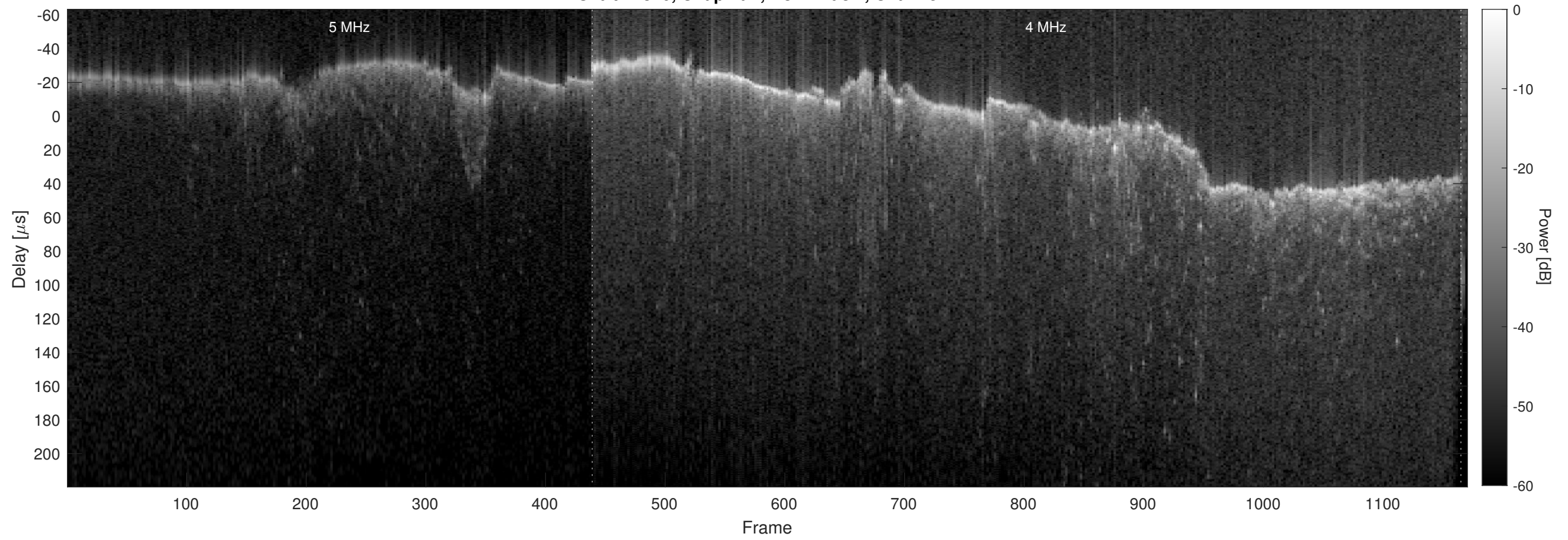
Orbit 21840, Chapman, No Window, Channel 2
