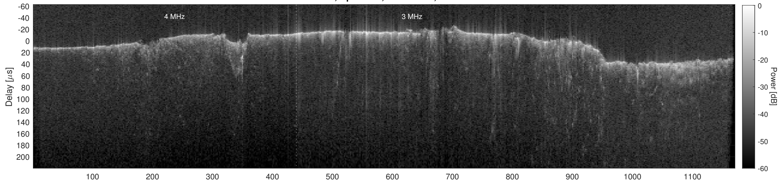
Orbit 21840, Cluttergram
