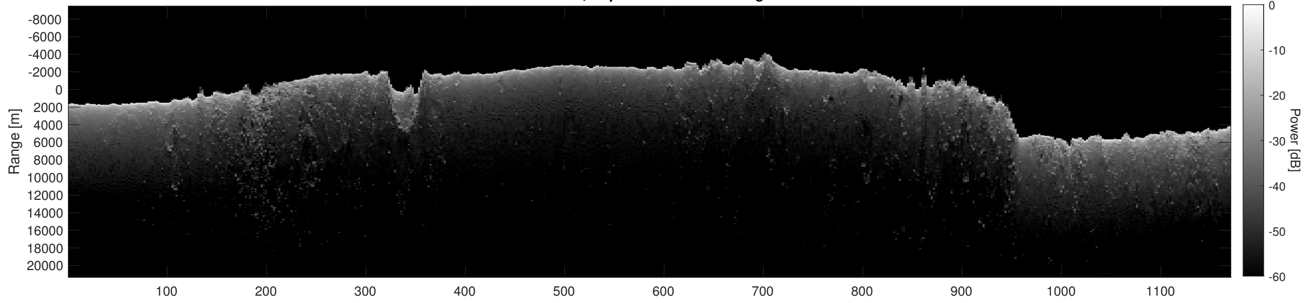
Orbit 21840, Depth-Corrected Cluttergram
