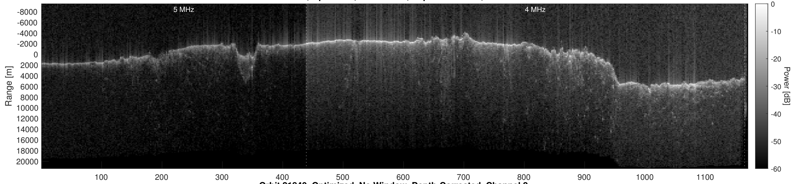
Orbit 21840, Optimized, No Window, Depth-Corrected, Channel 2
