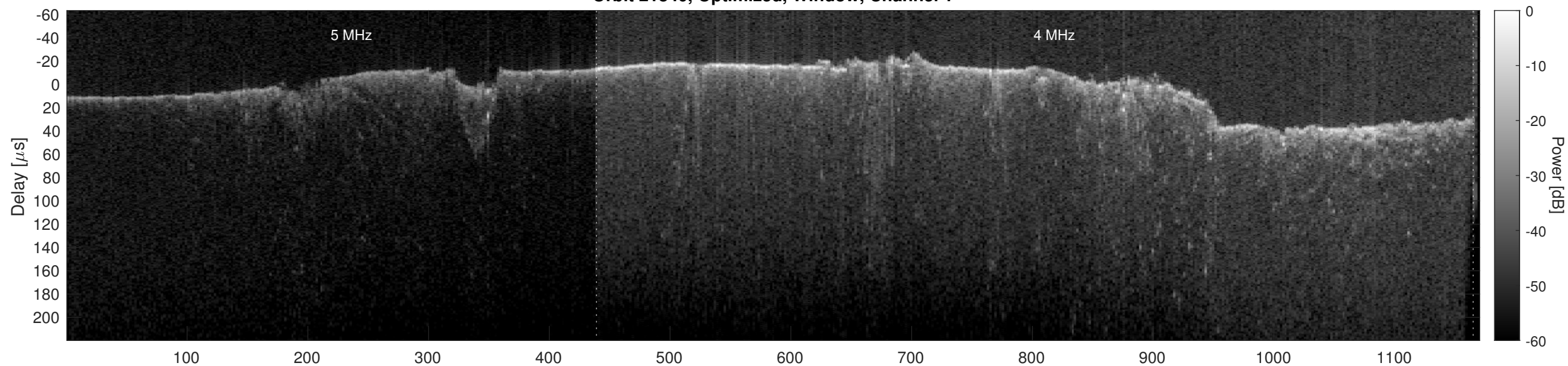
Orbit 21840, Optimized, Window, Channel 2
