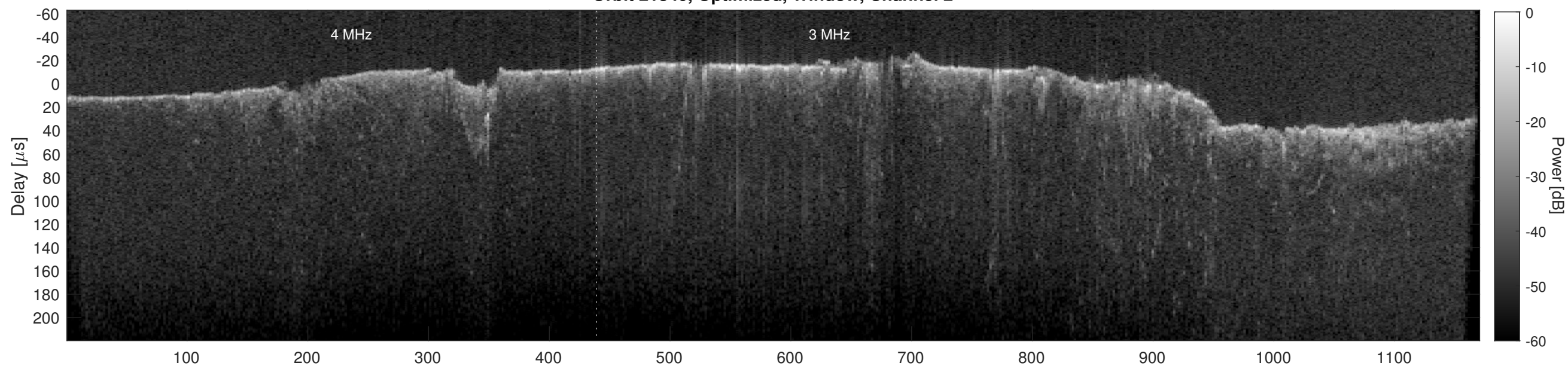
Orbit 21840, Cluttergram
