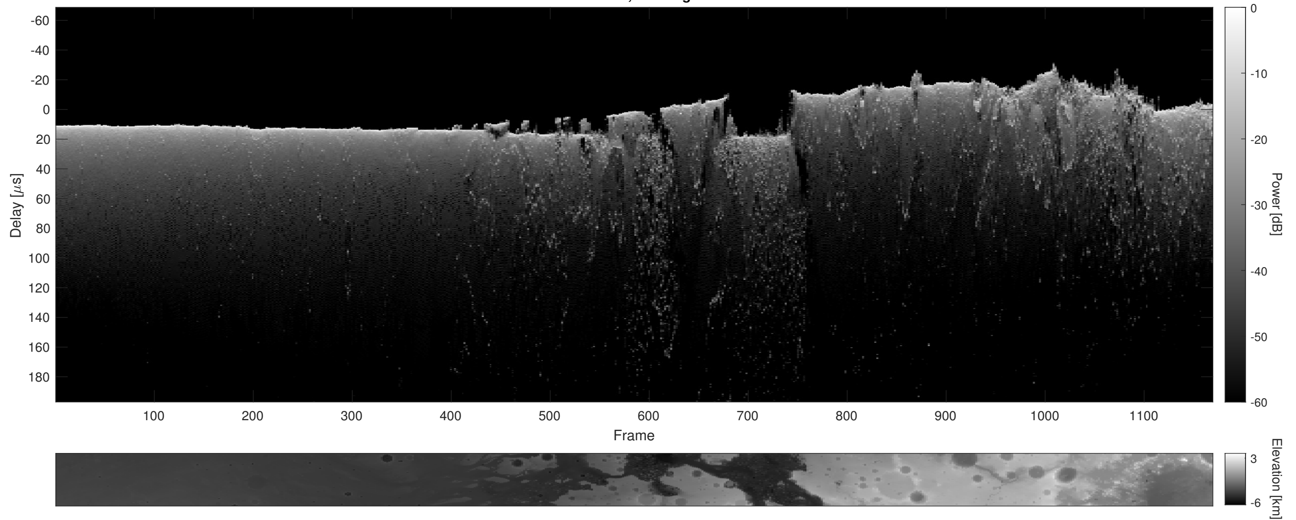
Orbit 21841, Cluttergram
