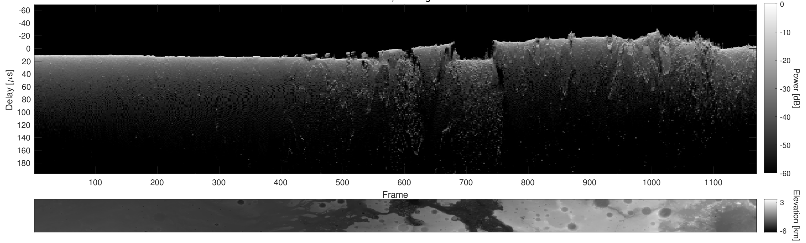
Orbit 21841, Cluttergram
