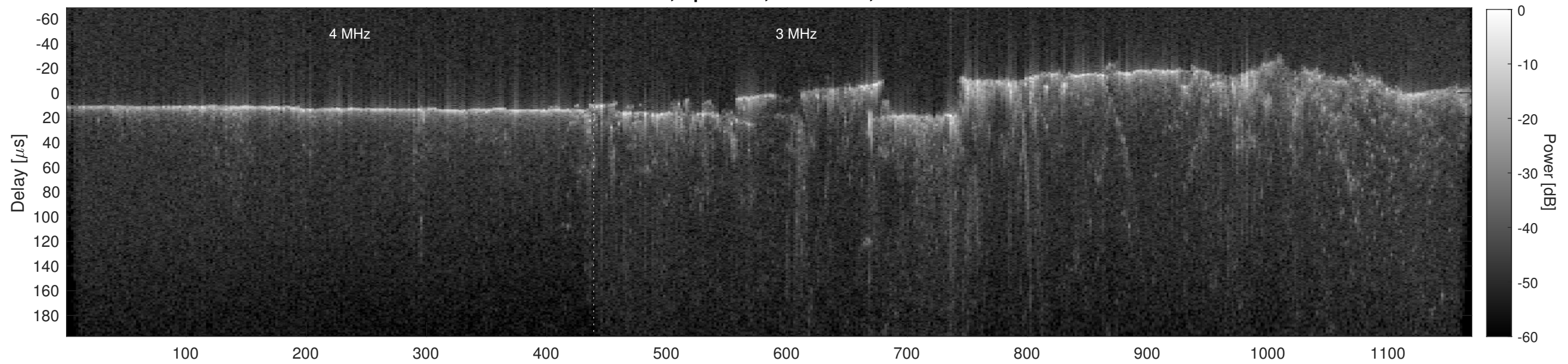
Orbit 21841, Cluttergram
