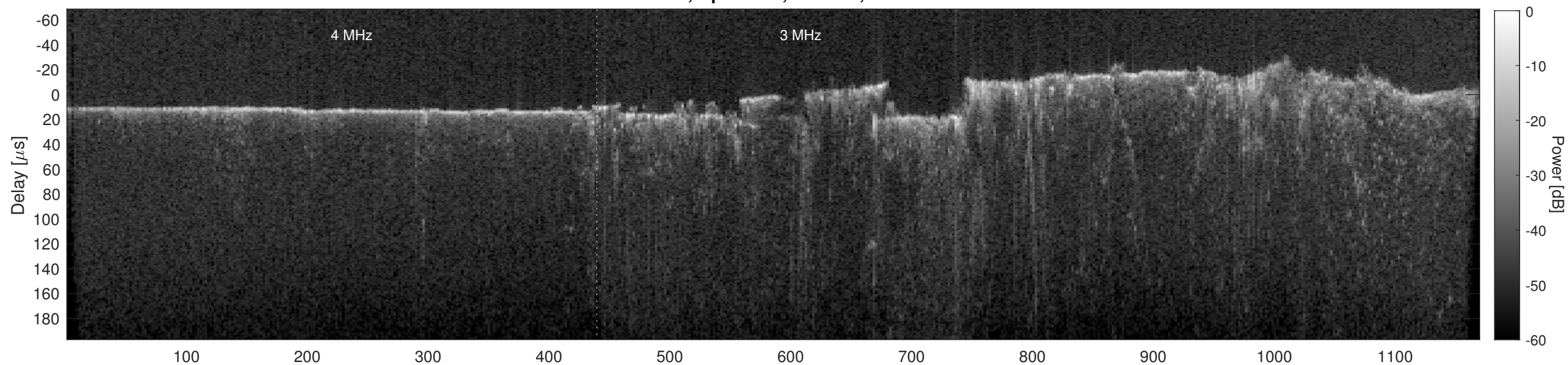
Orbit 21841, Cluttergram
