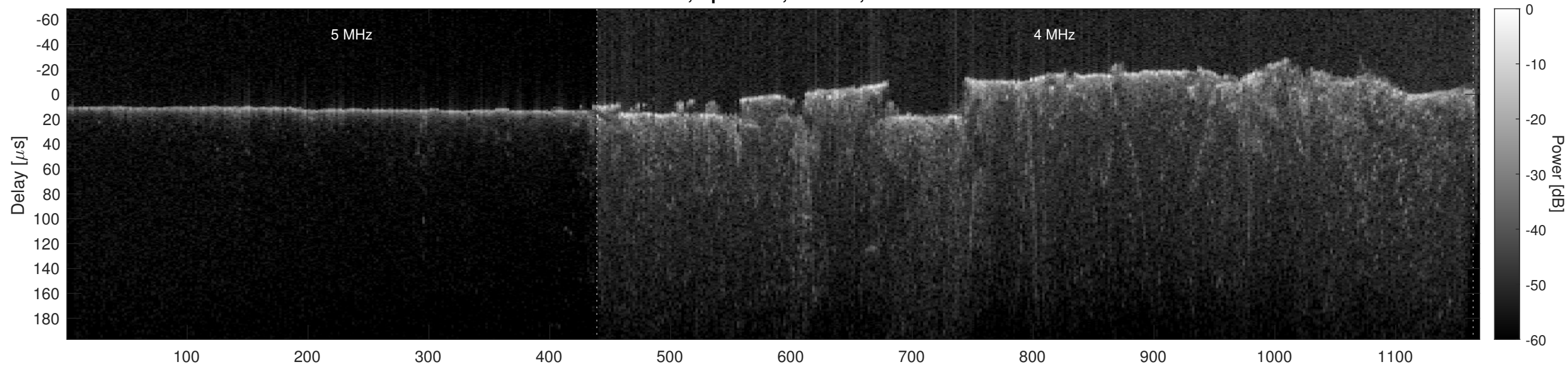
Orbit 21841, Optimized, Window, Channel 2
