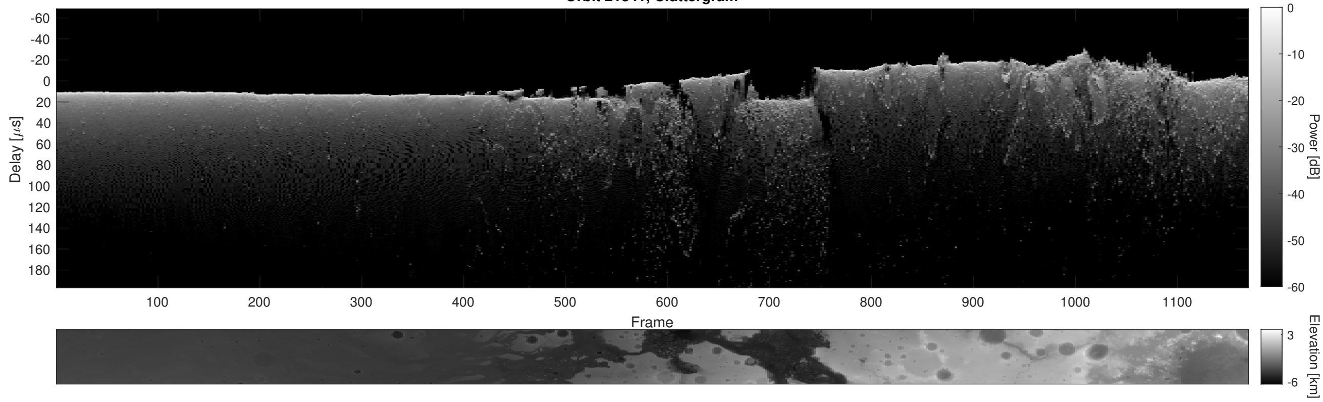
Orbit 21841, Cluttergram
