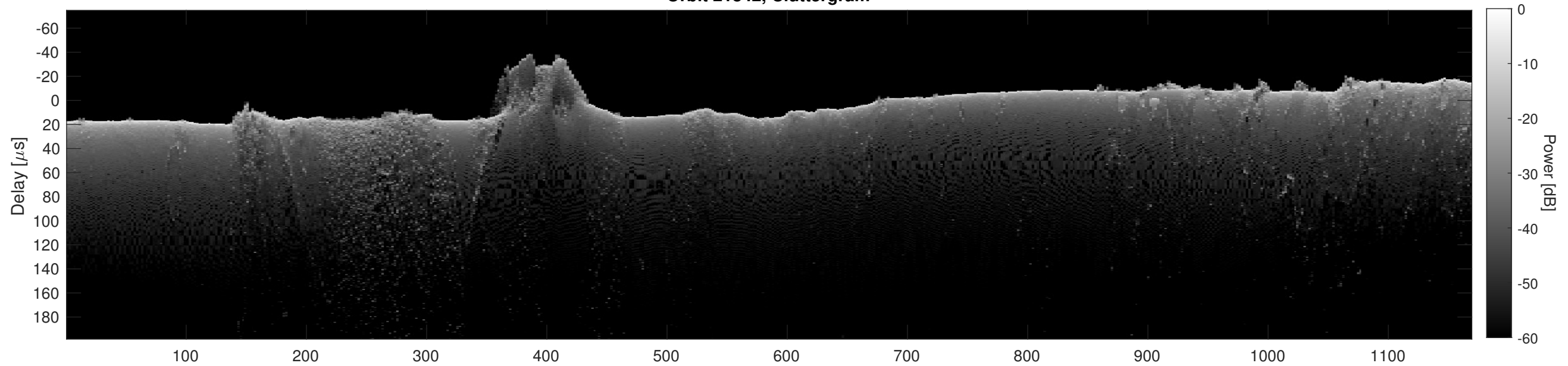
Orbit 21842, Cluttergram
