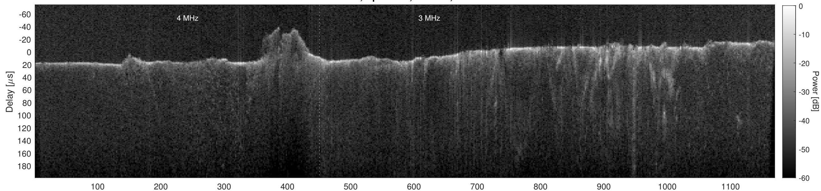
Orbit 21842, Cluttergram
