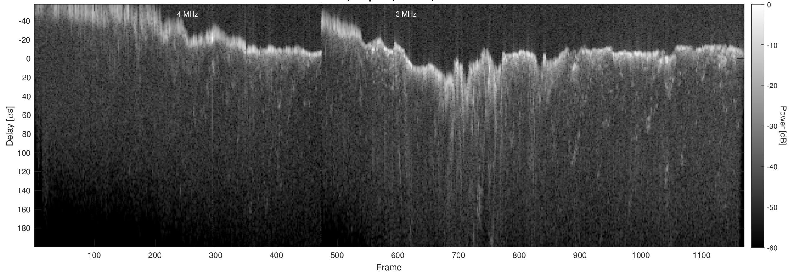
Orbit 21844, Chapman, Window, Channel 2
