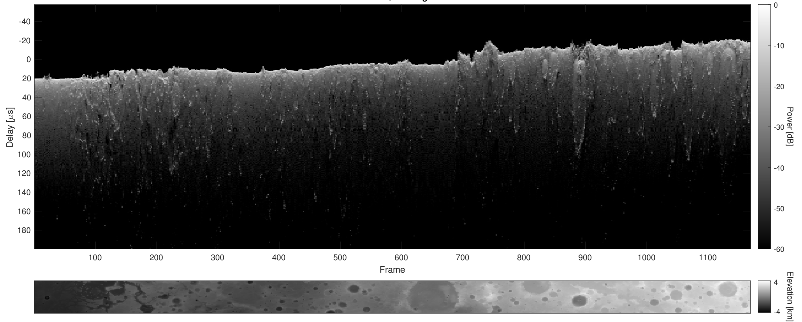
Orbit 21844, Cluttergram
