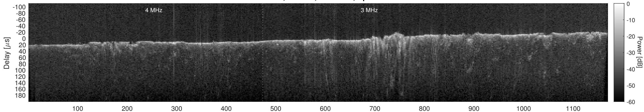
Orbit 21844, Cluttergram
