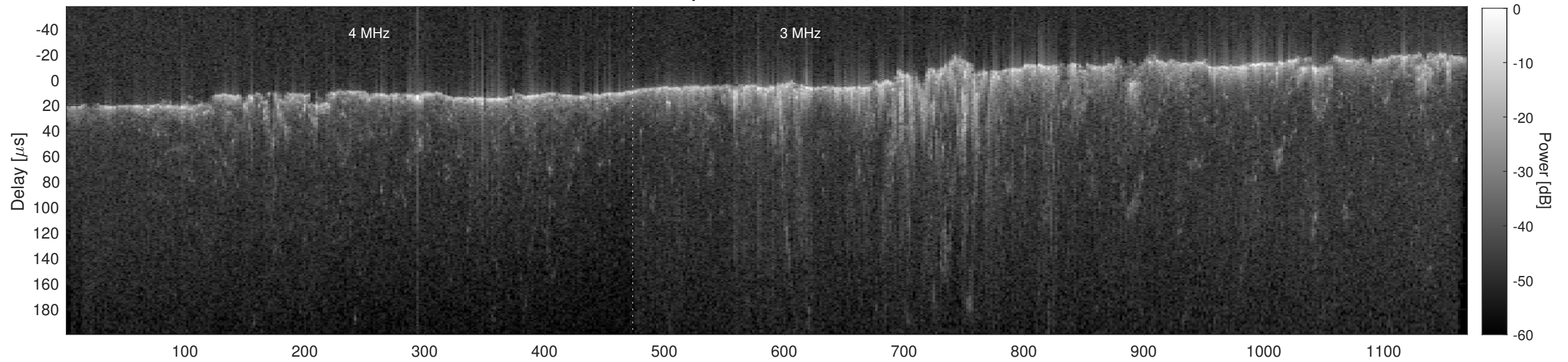
Orbit 21844, Cluttergram
