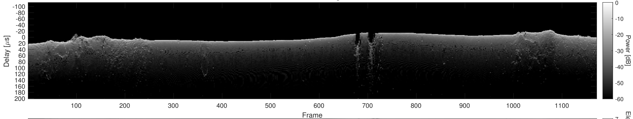
Orbit 21845, Cluttergram
