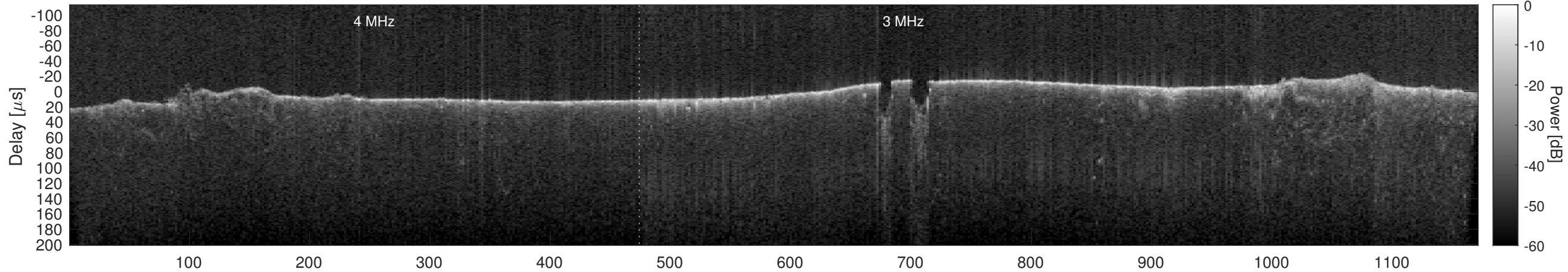
Orbit 21845, Cluttergram
