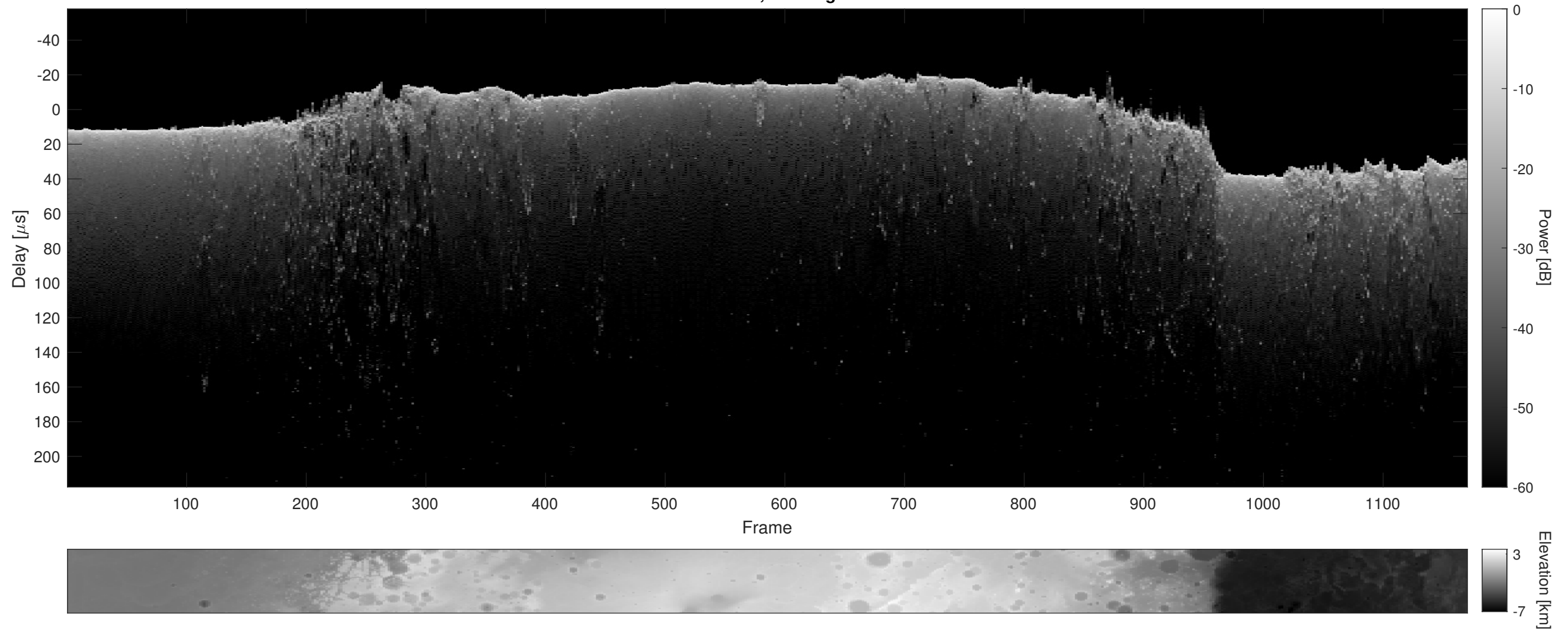
Orbit 21847, Cluttergram
