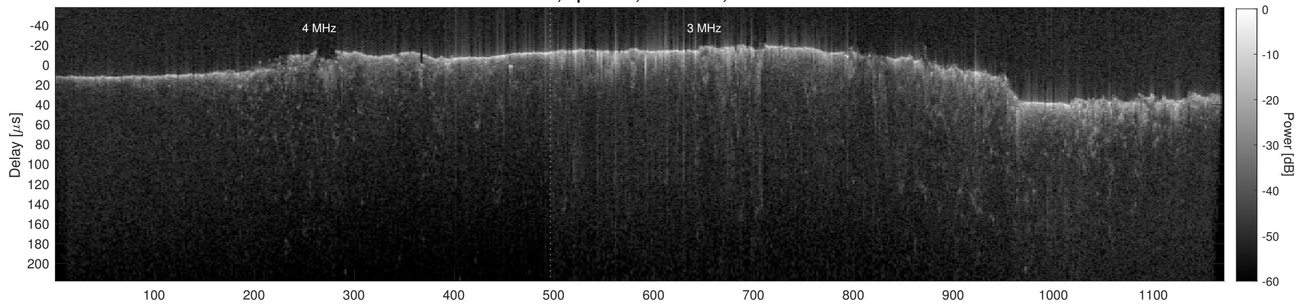
Orbit 21847, Cluttergram
