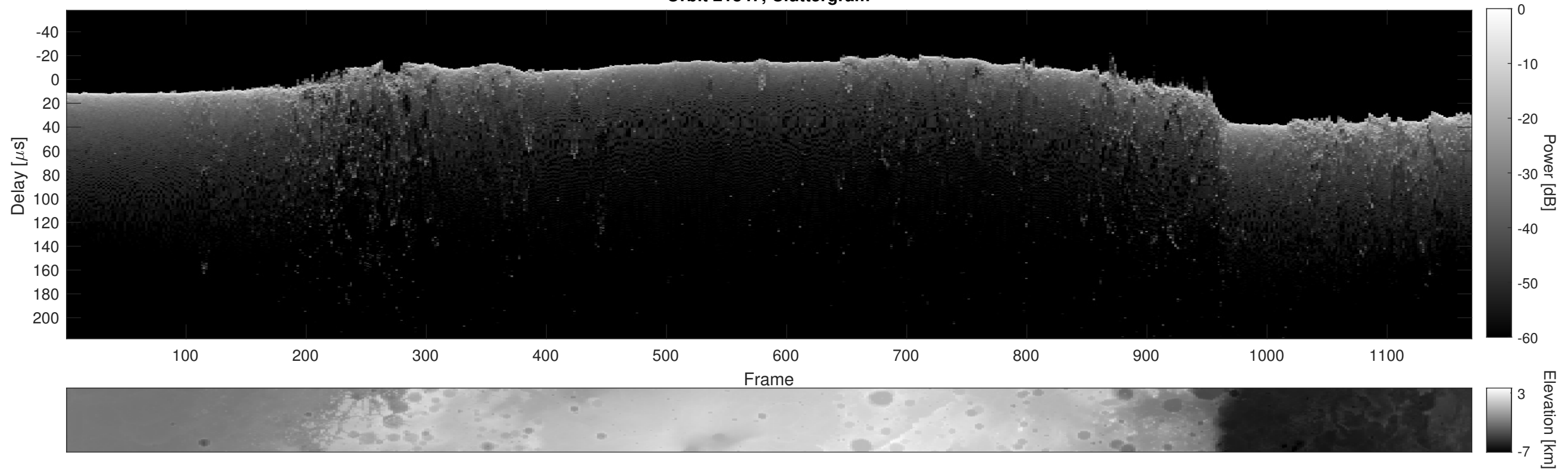
Orbit 21847, Cluttergram
