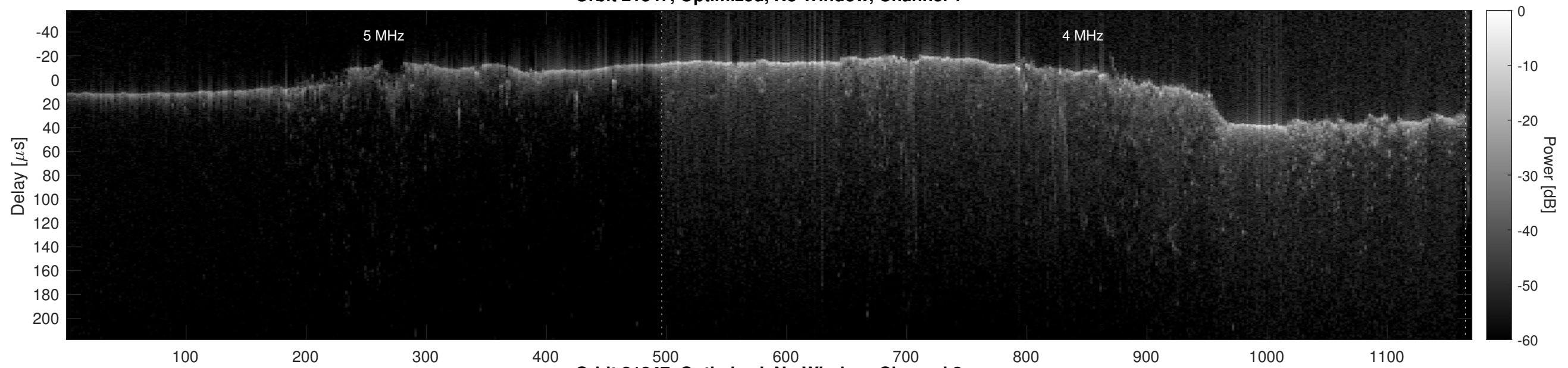
Orbit 21847, Optimized, No Window, Channel 2
