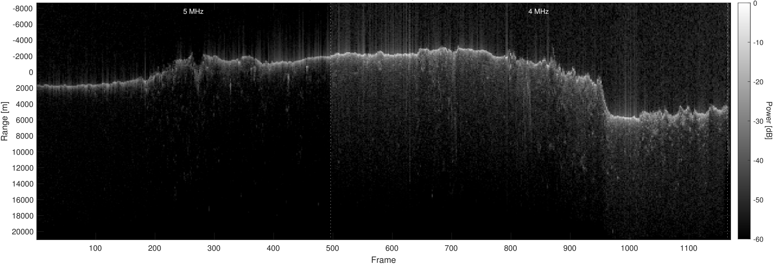
Orbit 21847, Optimized, No Window, Depth-Corrected, Channel 2
