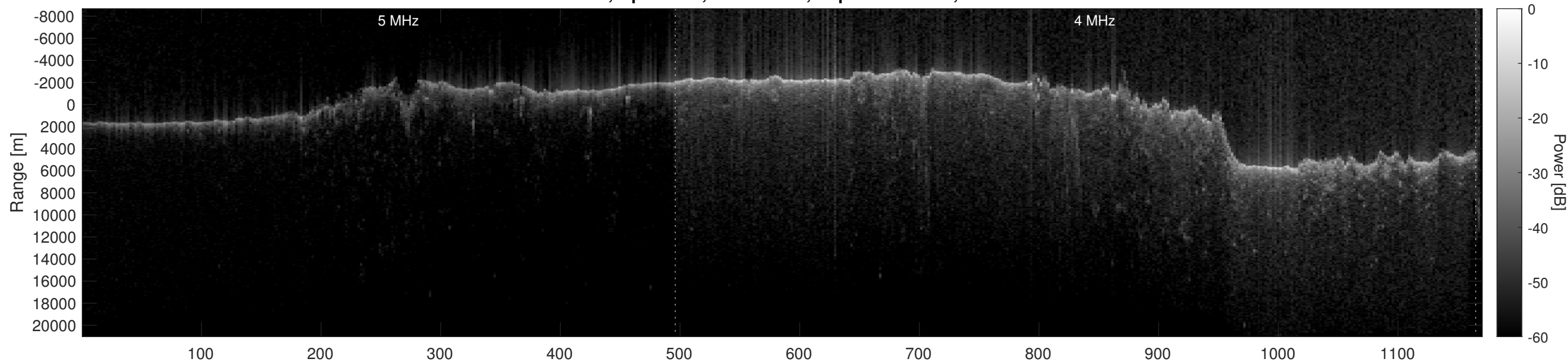
Orbit 21847, Optimized, No Window, Depth-Corrected, Channel 2
