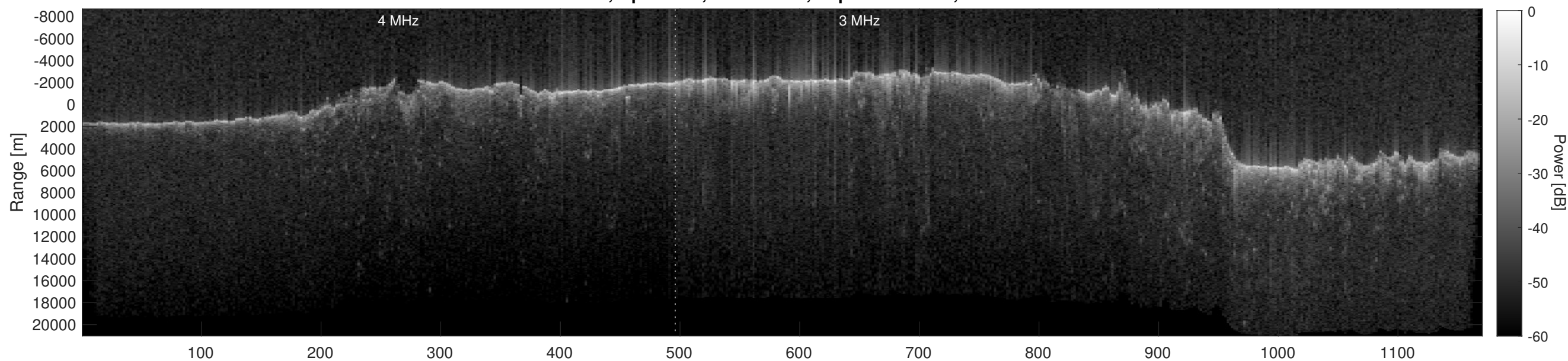
Orbit 21847, Depth-Corrected Cluttergram
