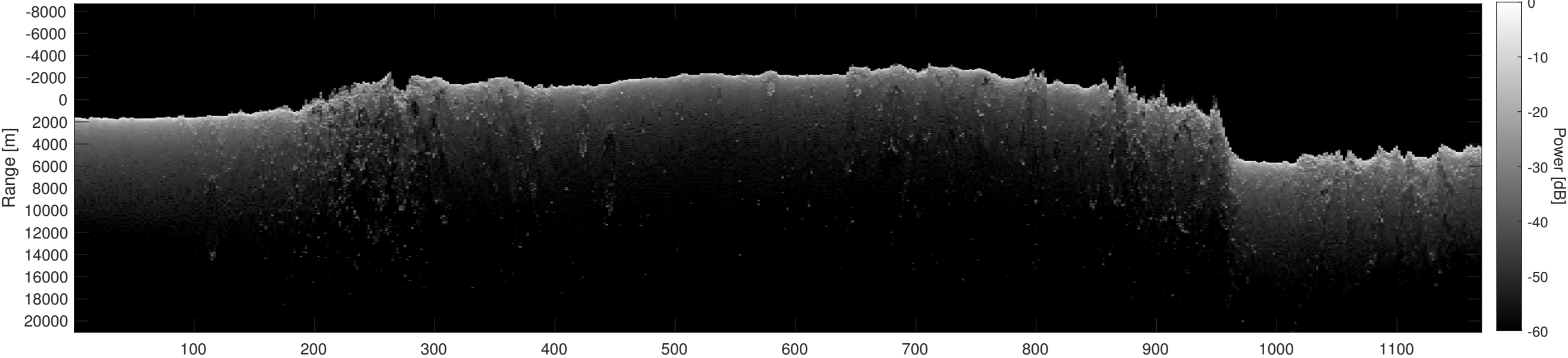
Orbit 21847, Depth-Corrected Cluttergram
