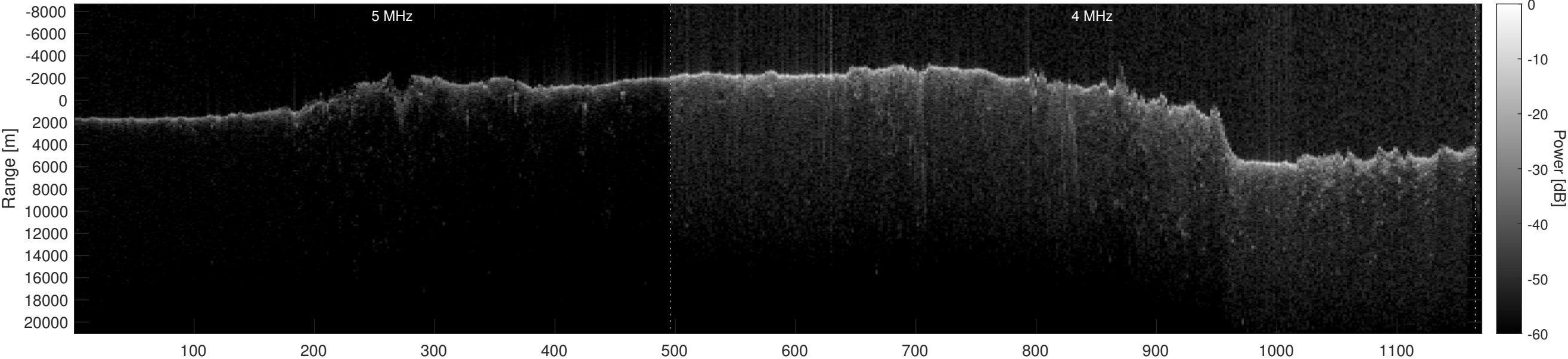
Orbit 21847, Optimized, Window, Depth-Corrected, Channel 2
