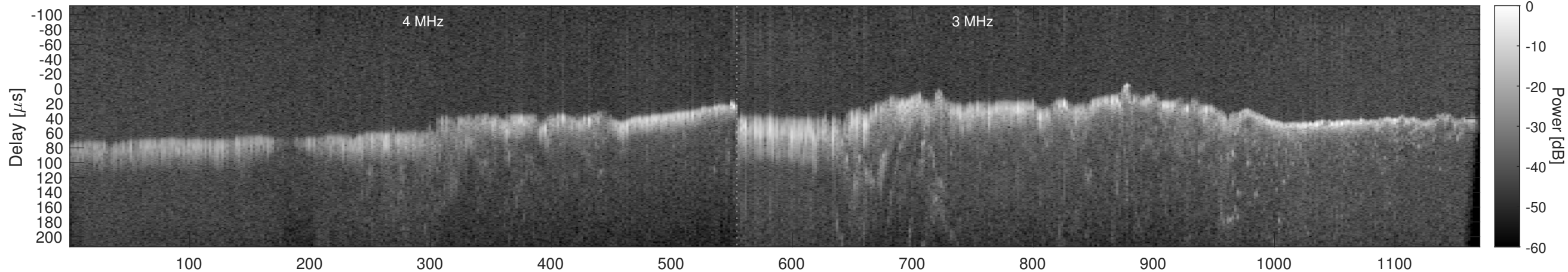
Orbit 21854, Window, Channel 2, Chapman
