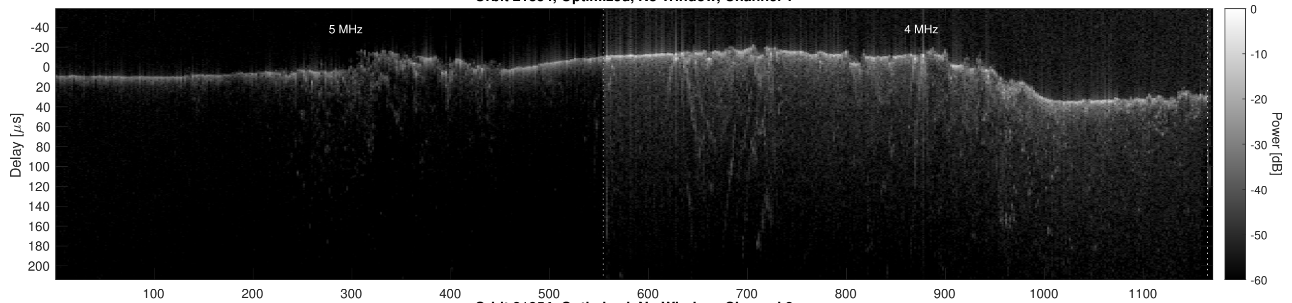
Orbit 21854, Optimized, No Window, Channel 2
