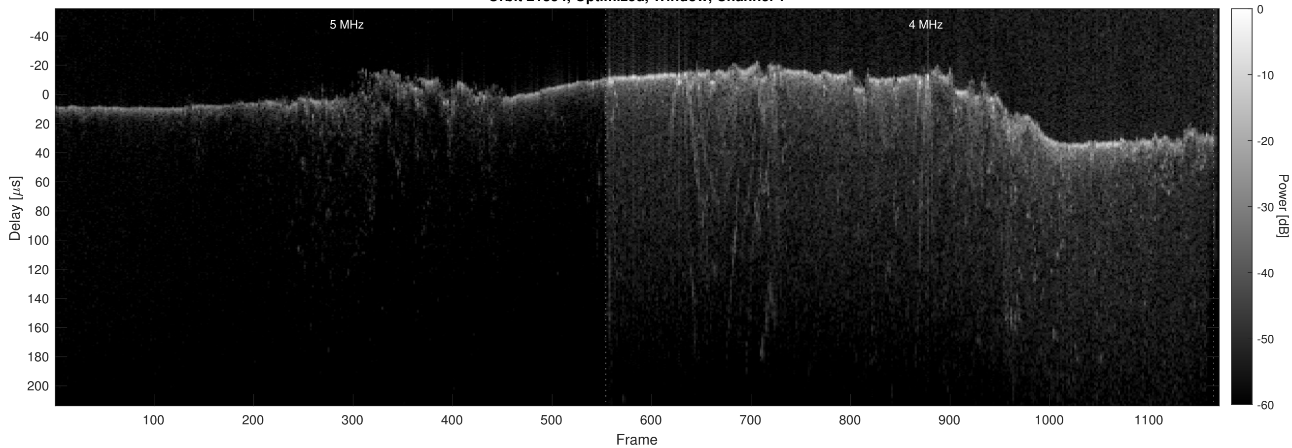
Orbit 21854, Optimized, Window, Channel 2
