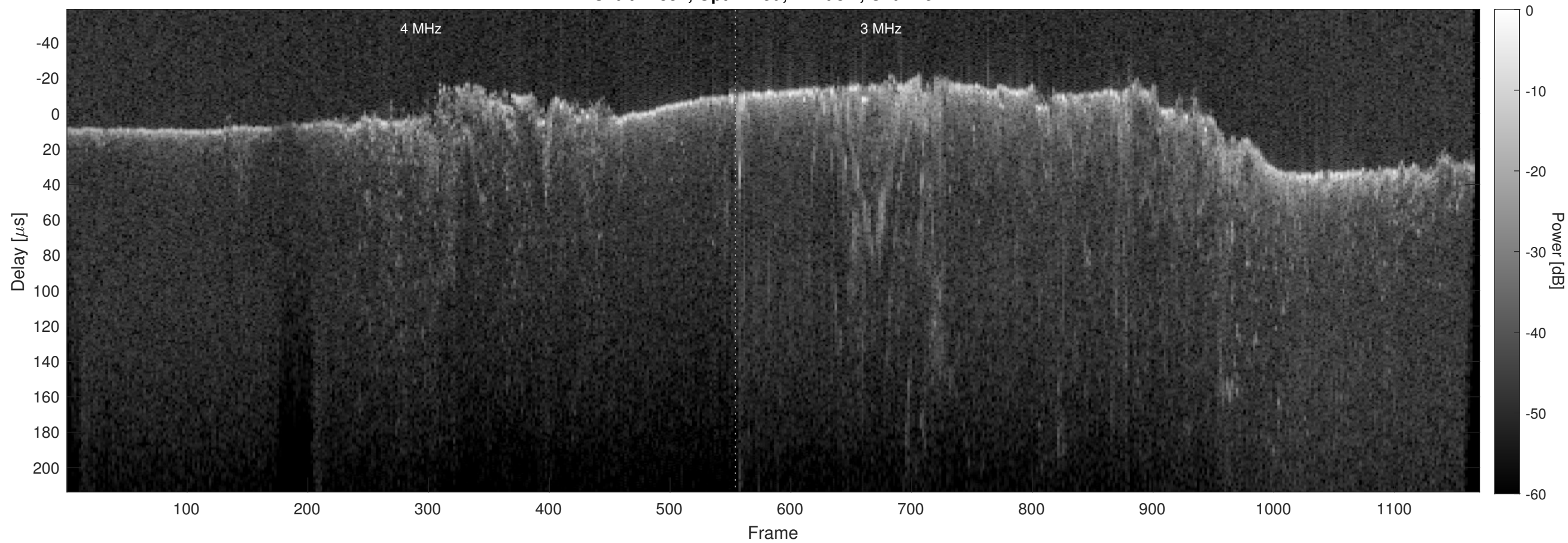
Orbit 21854, Optimized, Window, Channel 2
