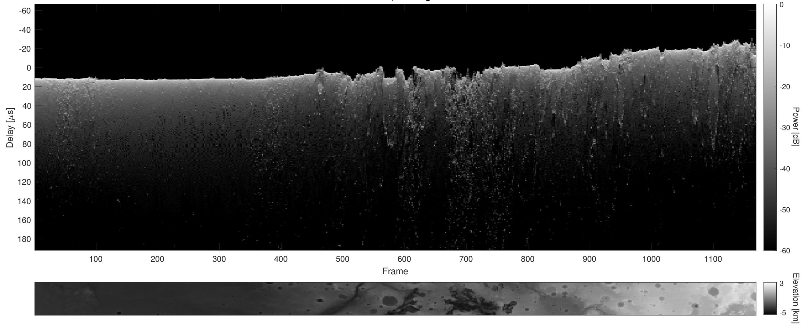
Orbit 21855, Cluttergram
