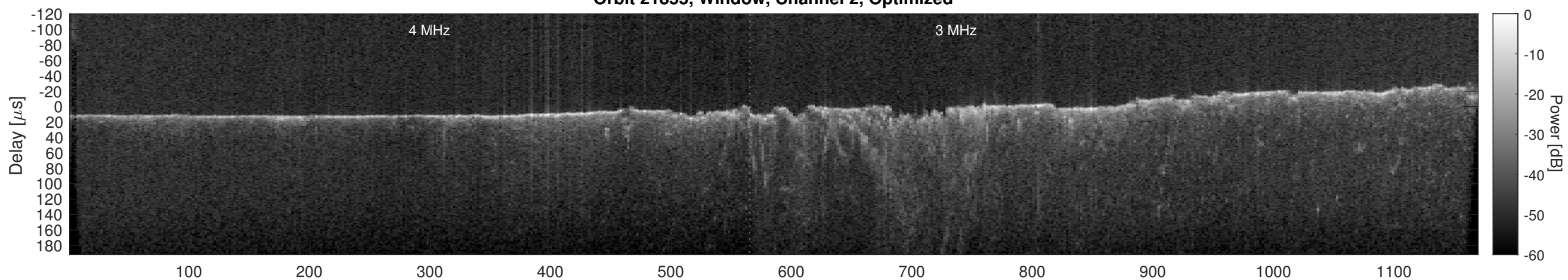
Orbit 21855, Cluttergram
