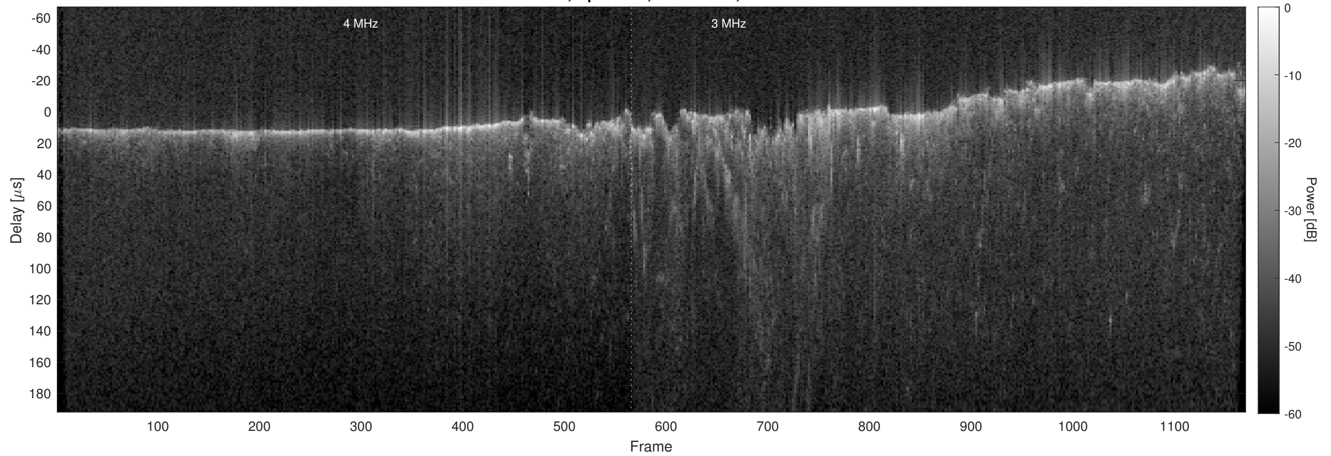
Orbit 21855, Optimized, No Window, Channel 2
