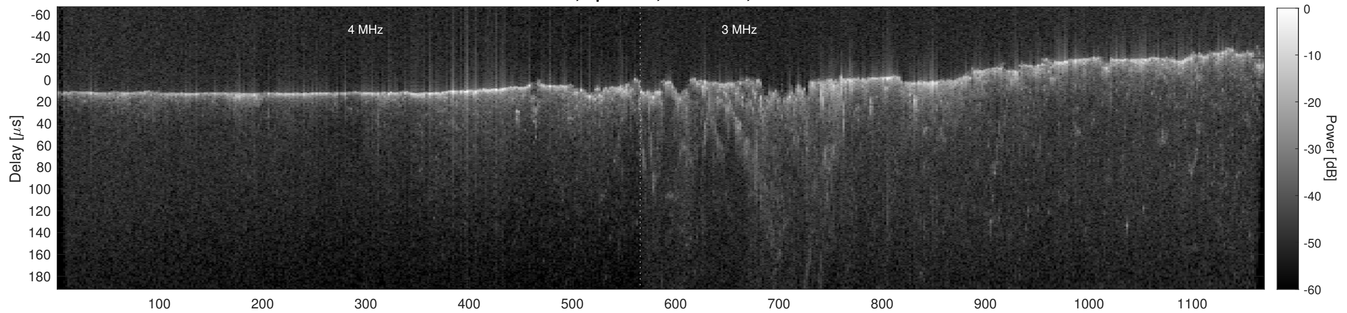
Orbit 21855, Cluttergram
