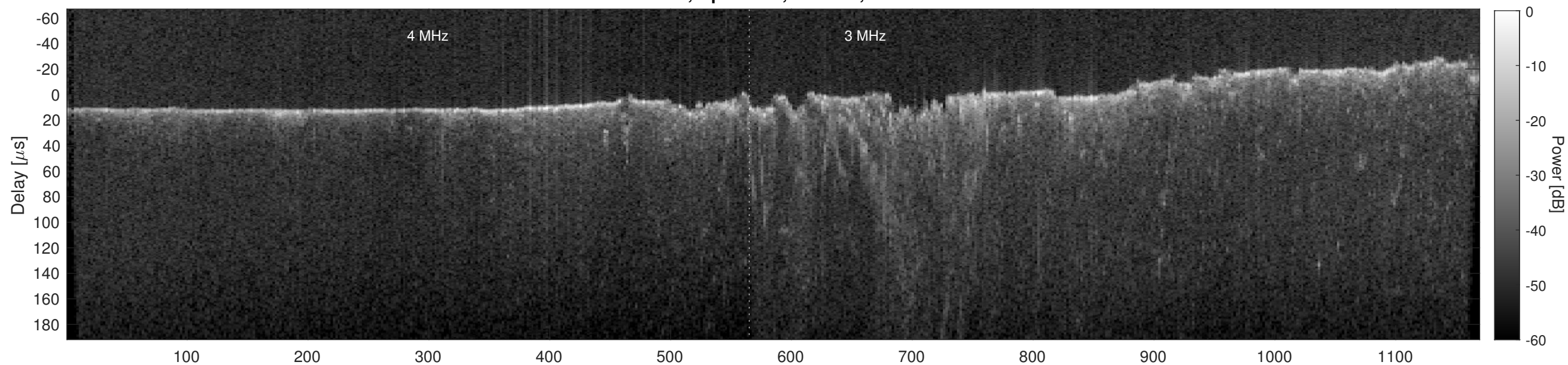
Orbit 21855, Cluttergram
