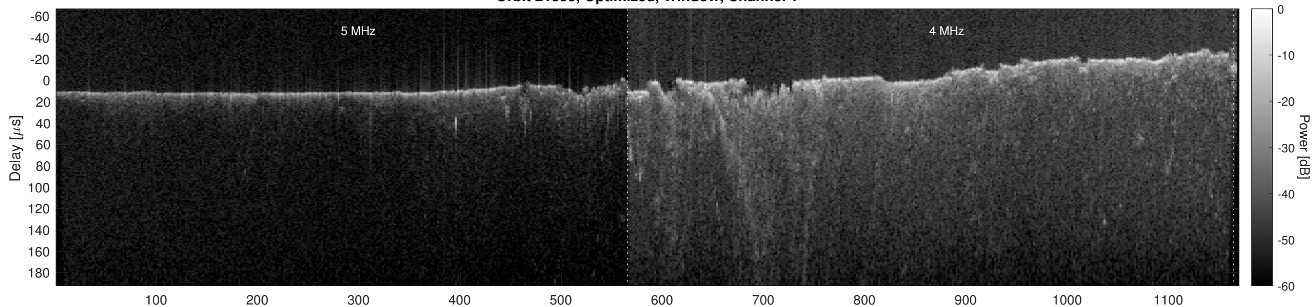
Orbit 21855, Optimized, Window, Channel 2
