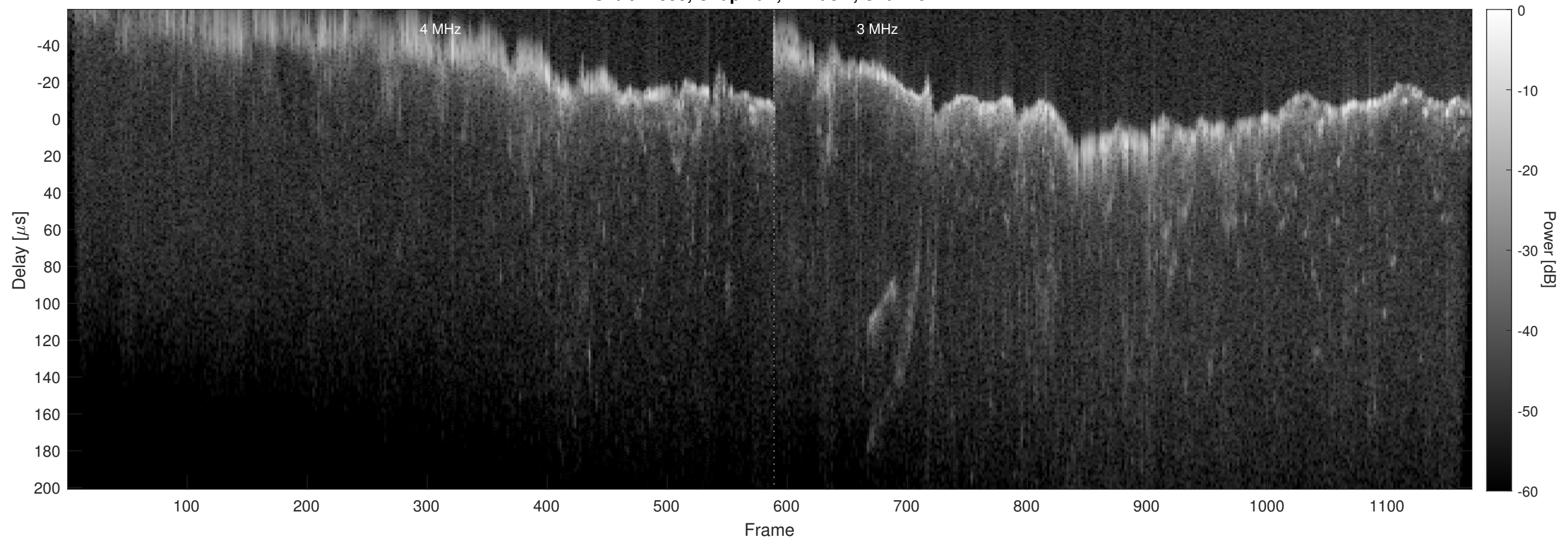
Orbit 21858, Chapman, Window, Channel 2
