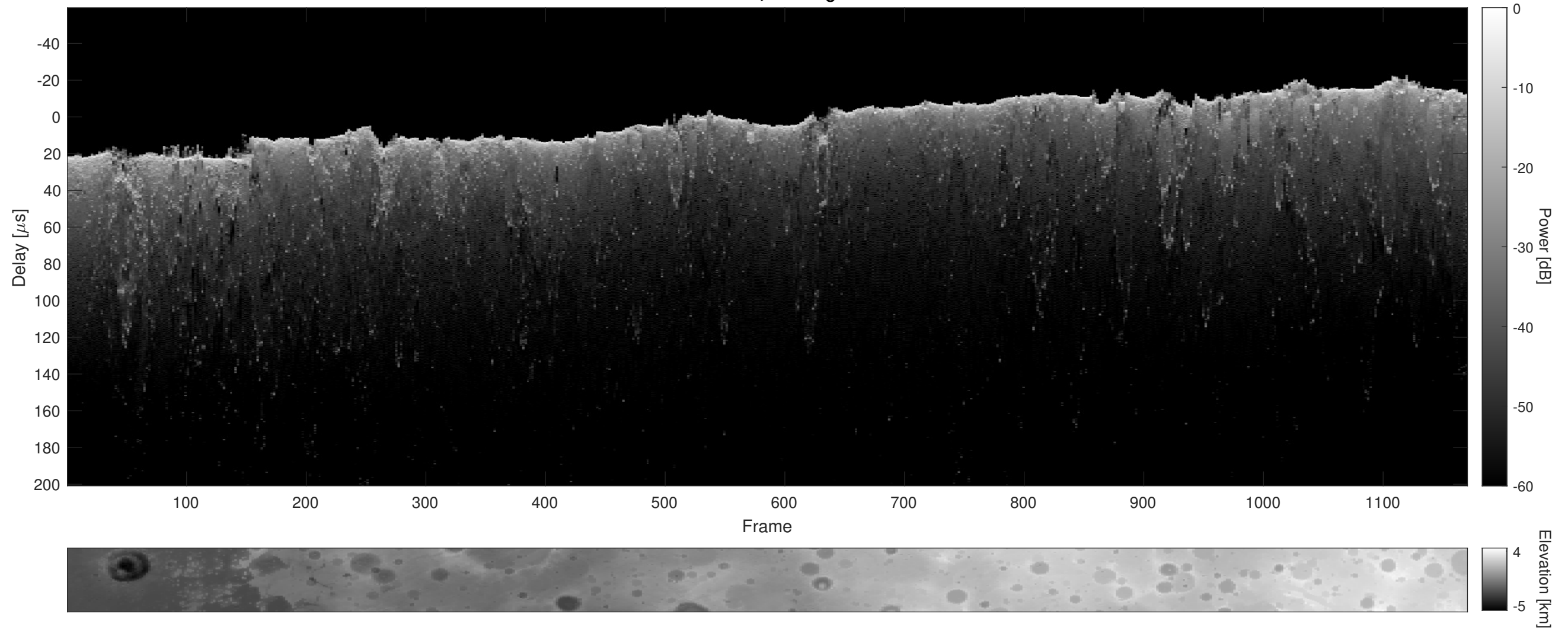
Orbit 21858, Cluttergram
