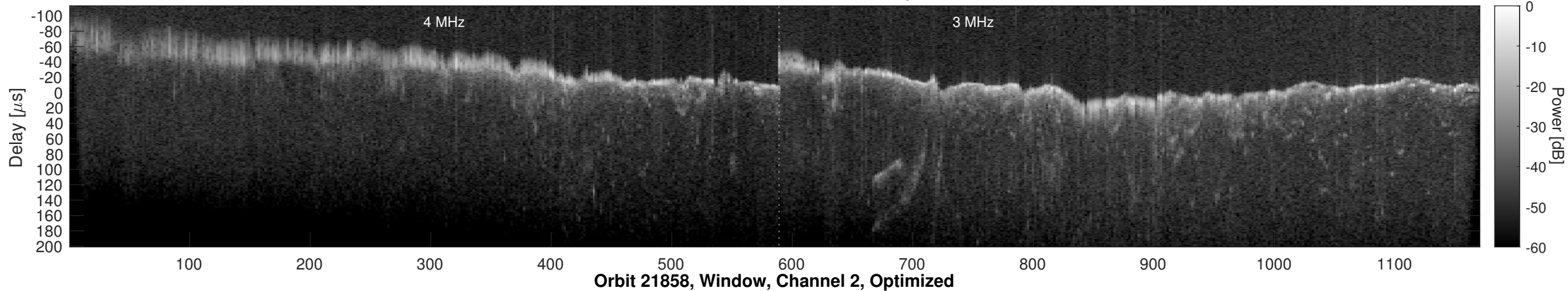
Orbit 21858, Window, Channel 2, Chapman
