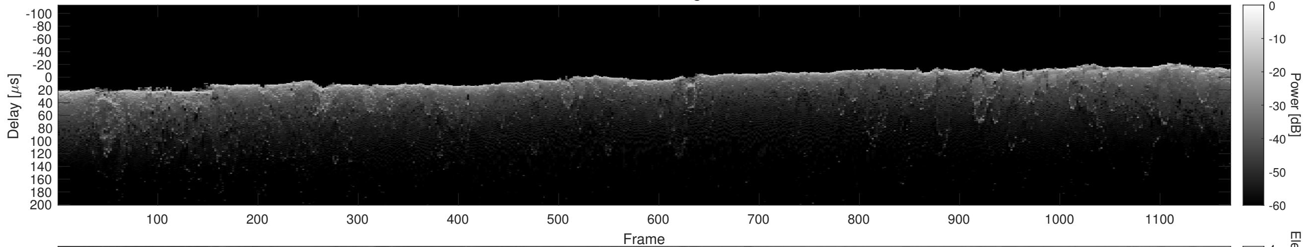
Orbit 21858, Cluttergram
