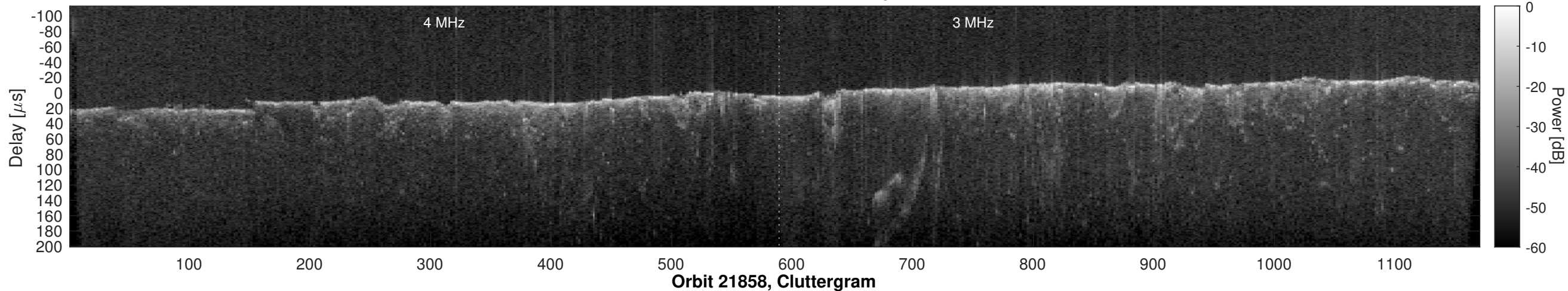
Orbit 21858, Window, Channel 2, Optimized
