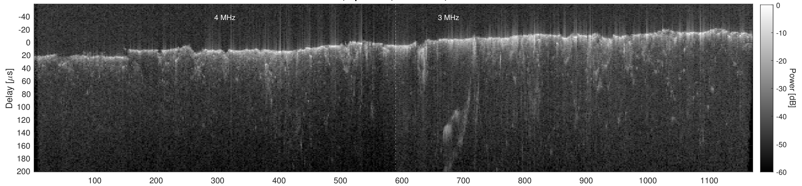
Orbit 21858, Cluttergram
