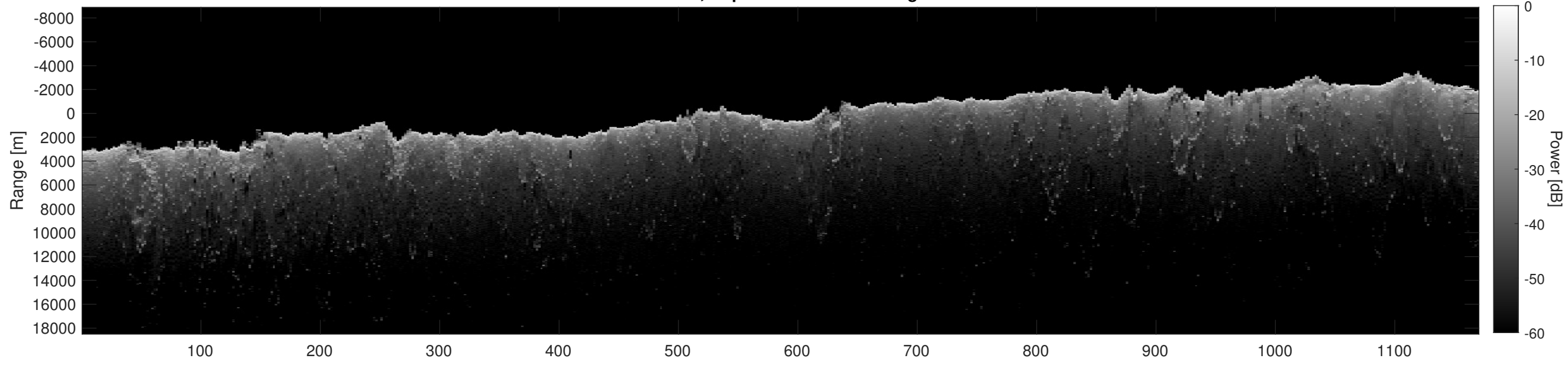
Orbit 21858, Depth-Corrected Cluttergram
