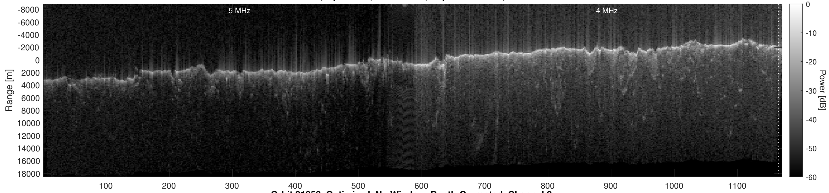
Orbit 21858, Optimized, No Window, Depth-Corrected, Channel 2
