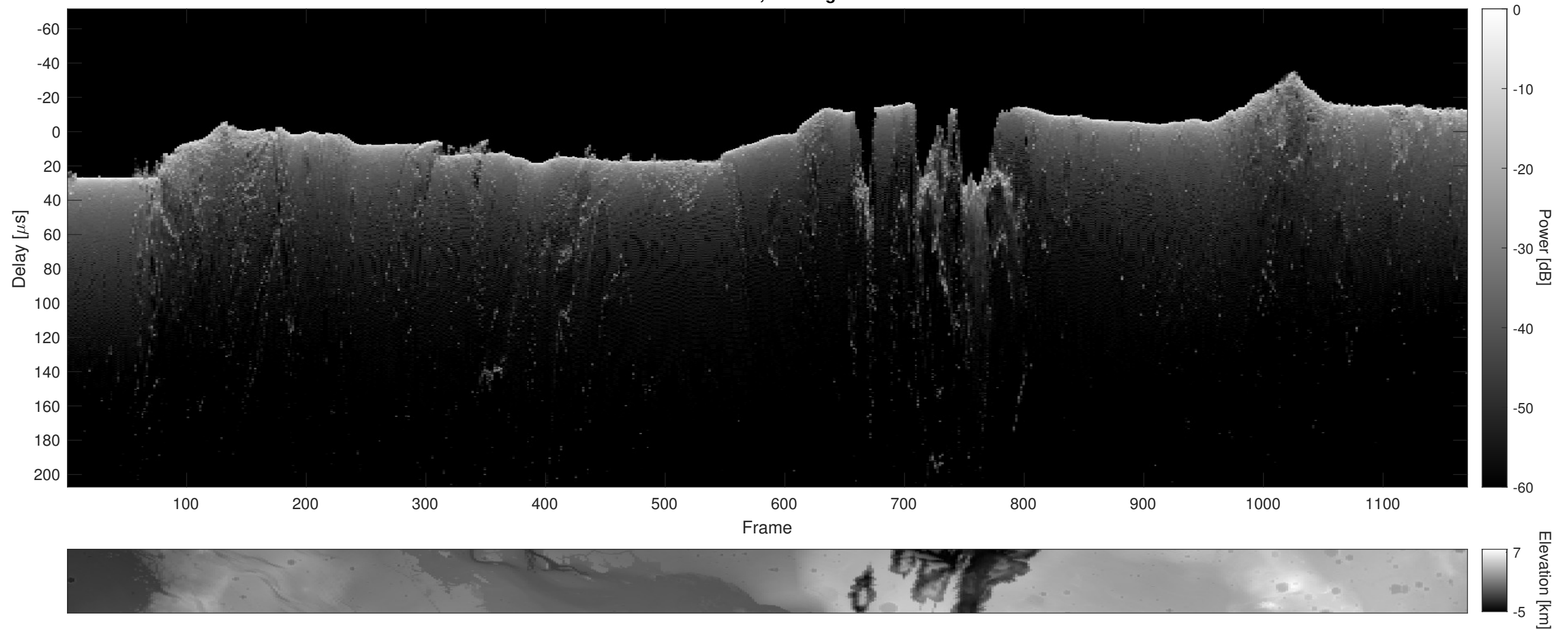
Orbit 21859, Cluttergram
