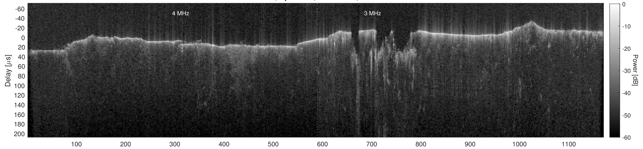
Orbit 21859, Cluttergram
