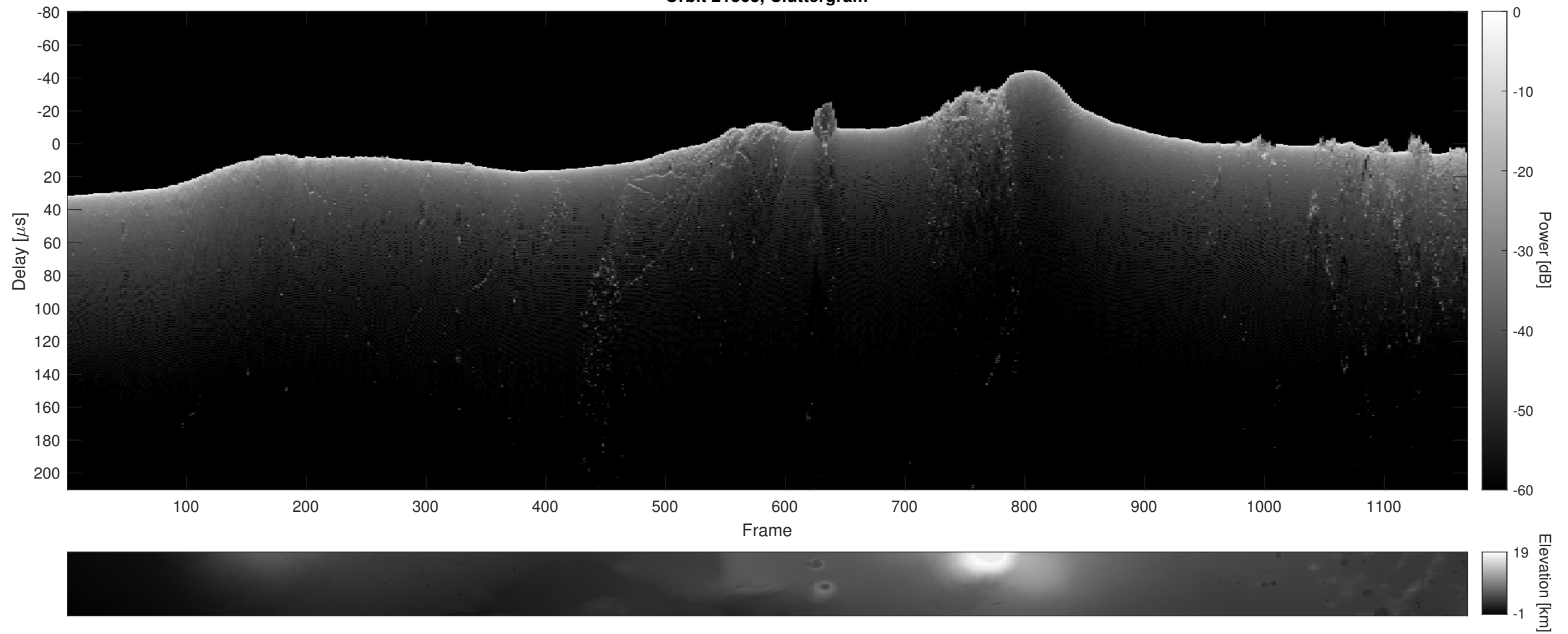
Orbit 21863, Cluttergram
