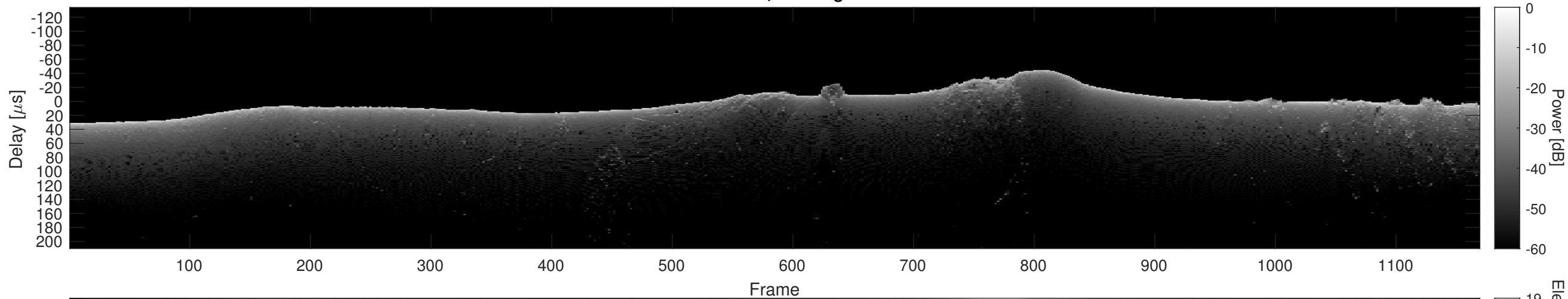
Orbit 21863, Cluttergram
