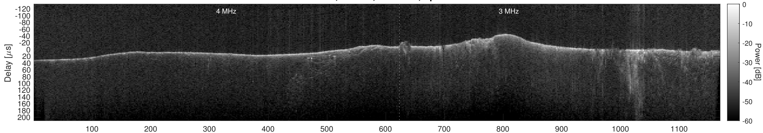
Orbit 21863, Cluttergram
