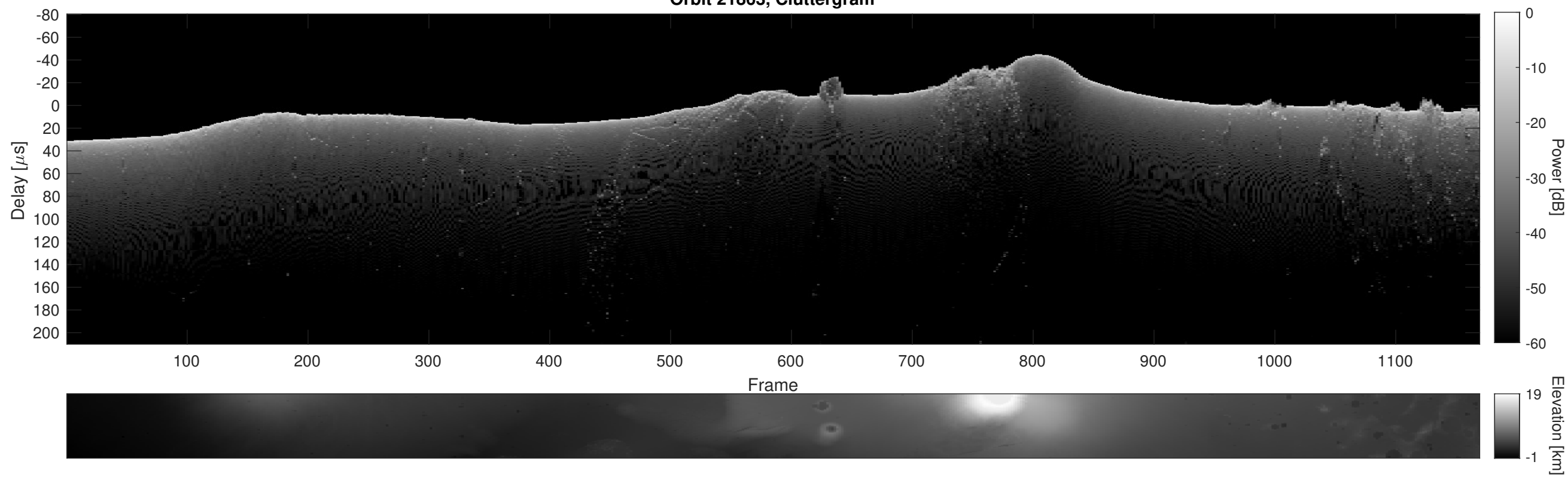
Orbit 21863, Cluttergram
